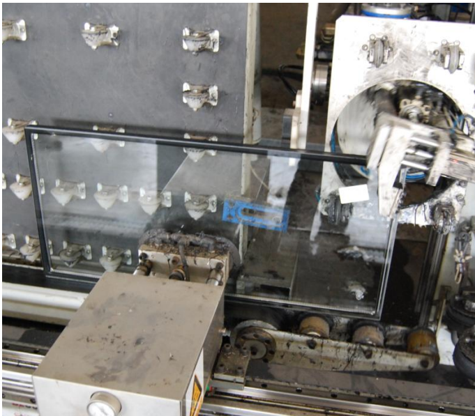
7. Double size glazed with structural tape
